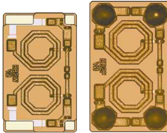
SCI-301W (Wirebond)
