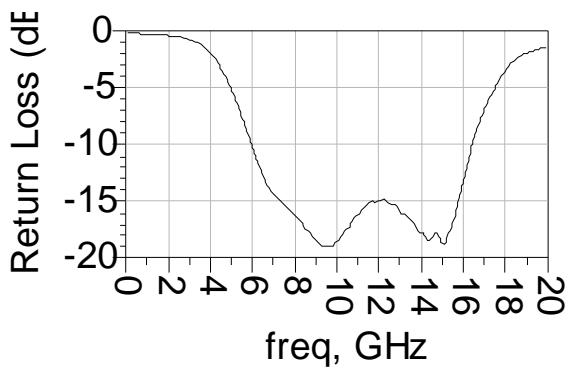
SCI-114W (Wirebond)
