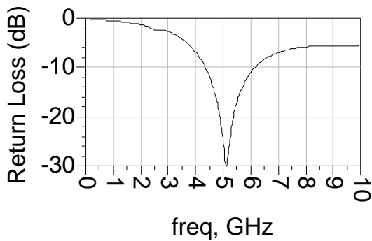
SCI-112W (Wirebond)
