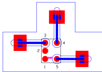
SCI-109F (Flip Chip)
