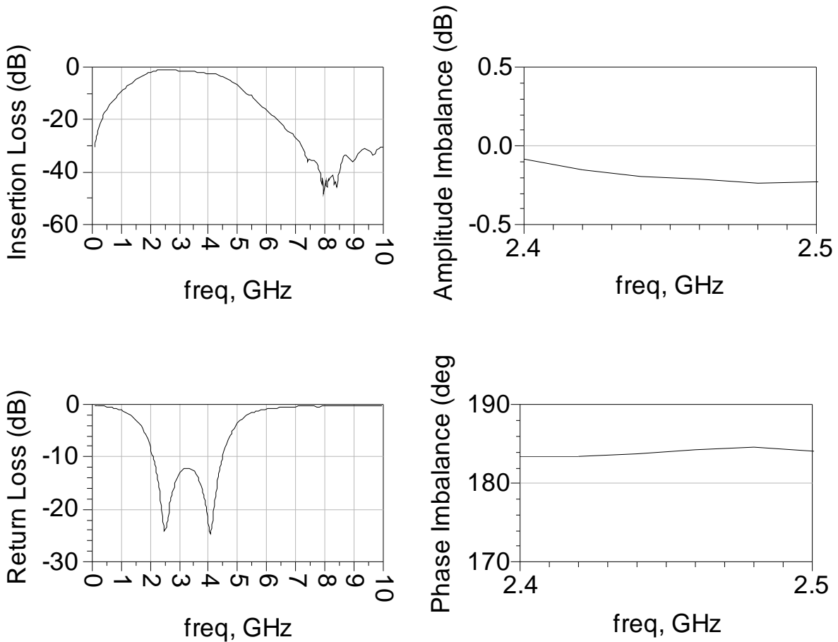
SCI-109W (Wirebond)
