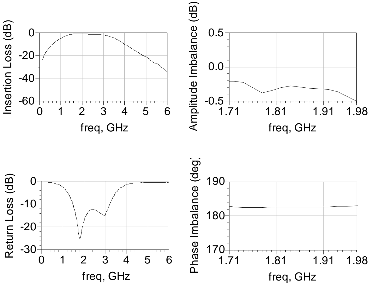
SCI-107W (Wirebond)
