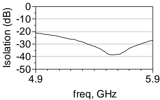
SCI-802W (Wirebond)
