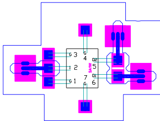
SCI-802W (Wirebond)
