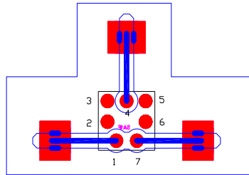
SCI-802F (Flip Chip)
