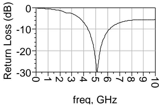
SCI-112W (Wirebond)
