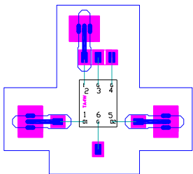
SCI-112W (Wirebond)
