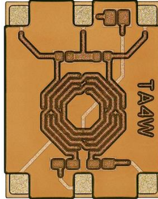
SCI-112W (Wirebond)
