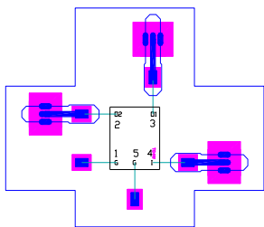
SCI-108W (Wirebond)
