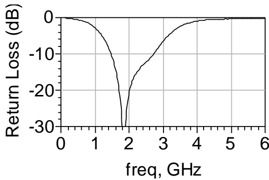
SCI-108W (Wirebond)
