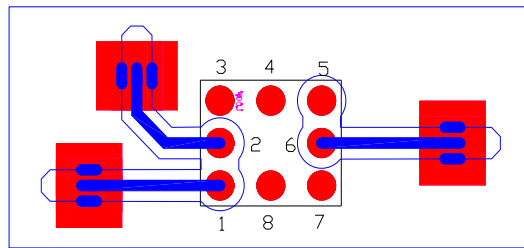
SCI-702F (Flip Chip)
