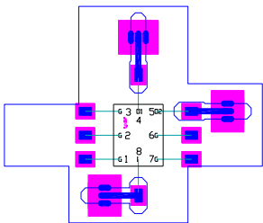
SCI-702W (Wirebond)
