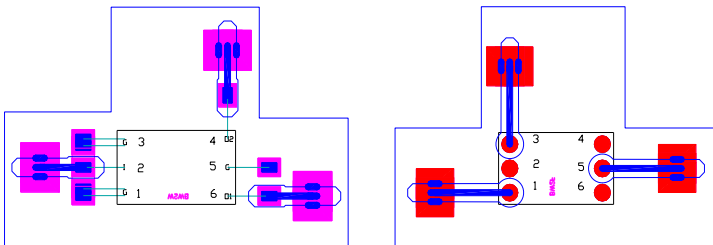
SCI-601W (Wirebond)
