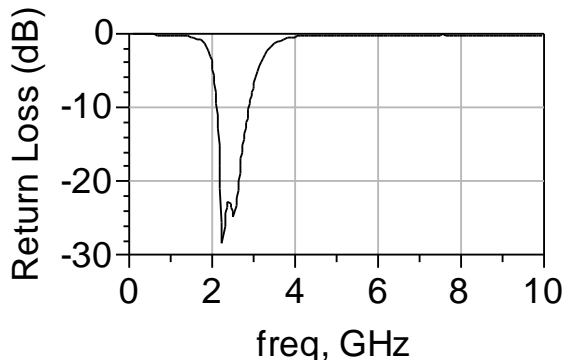
SCI-601W (Wirebond)
