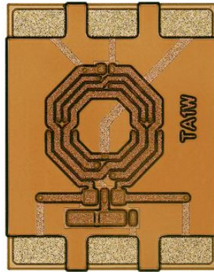
SCI-111W (Wirebond)
