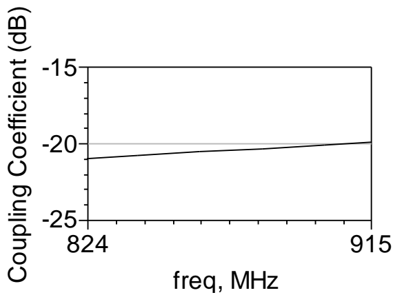
SCI-701W (Wirebond)
