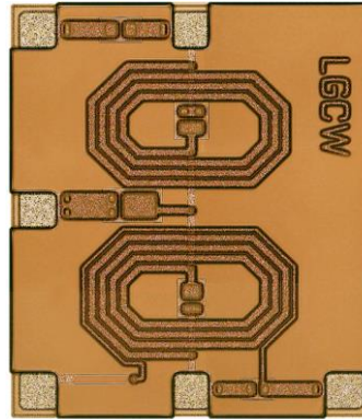
SCI-701W (Wirebond)
