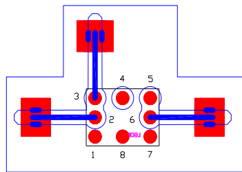
SCI-701F (Flip Chip)
