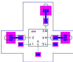
SCI-701W (Wirebond)
