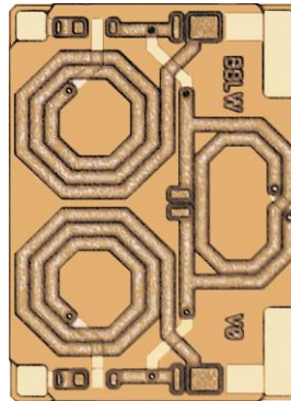
SCI-305W (Wirebond)
