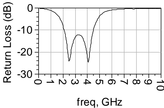
SCI-109W (Wirebond)
