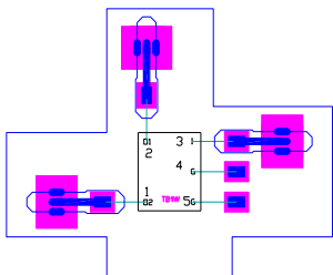
SCI-109W (Wirebond)
